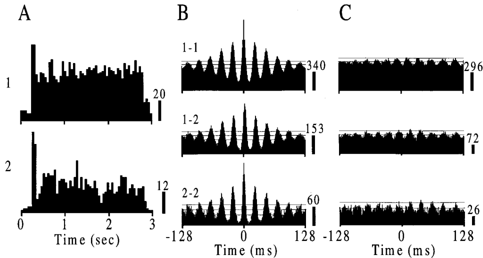
Figure 5. Stimulus-Evoked, Synchronized Oscillatory Activity in Striate Cortex of an Alert Macaque Monkey
